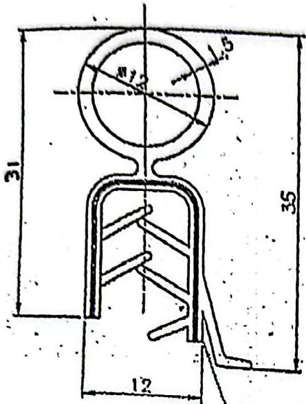
STEEL SPRING CORE
