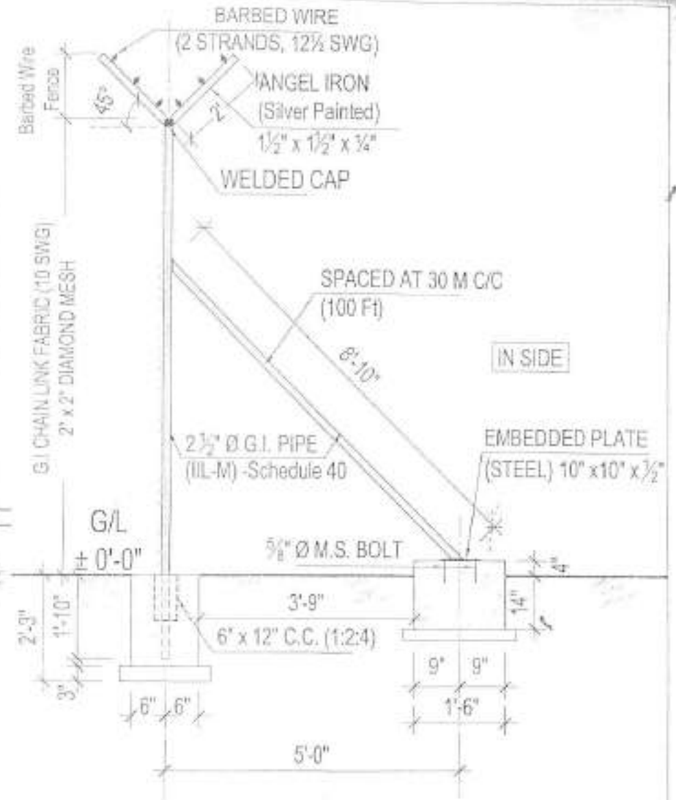
X-SECTION & REINF: DETAIL FOR FENCING WALL
