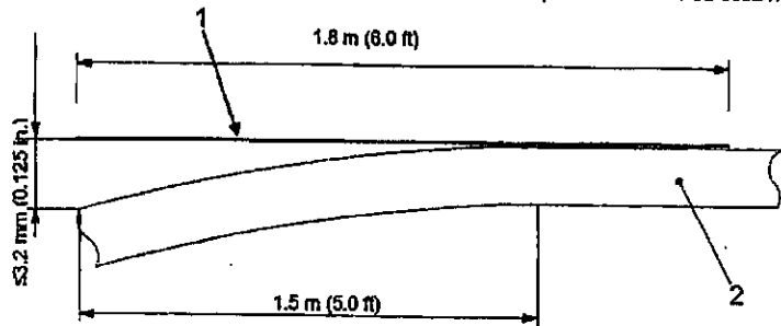
Figure 2—Measuring End Straightness
