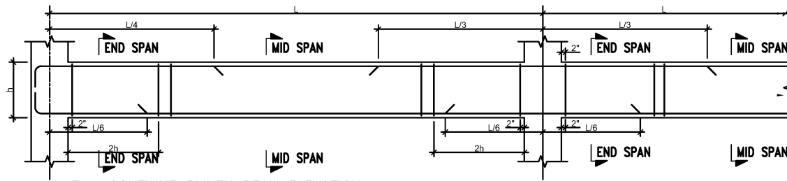
Typ. CONTINUE PLINTH BEAM ELEVATION
