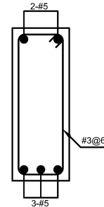
RB-3 (MID SPAN) (9"x 24")
