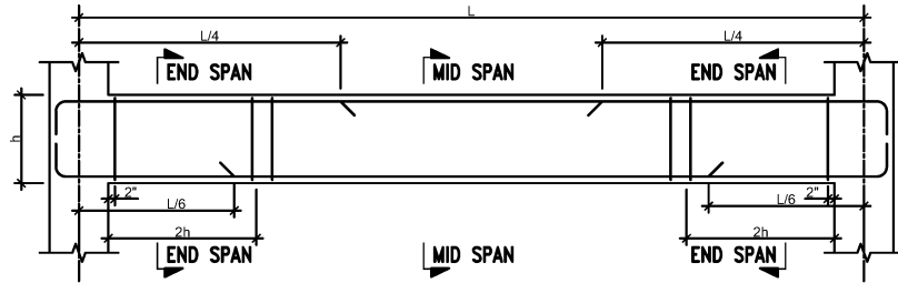
Typ. BEAM ELEVATION
