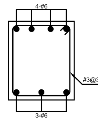
RB-4 (END SPAN) INVERTED (15"x 18")
