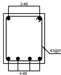
RB-1 (MID SPAN) INVERTED (15"x 18")
