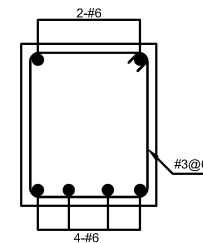
RB-4 (MID SPAN) INVERTED (15"x 18")
