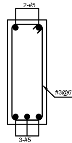
PB-1 (MID SPAN) (9"x 24")
