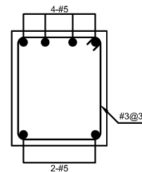
RB-2 (END SPAN) INVERTED (15"x 18")
