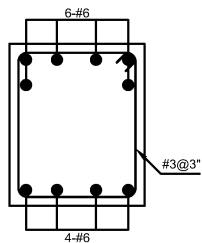
RB-1 (END SPAN) INVERTED (15"x 18")
