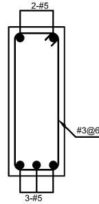
B-1 (MID SPAN) (9"x 24")
