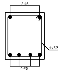
RB-2 (MID SPAN) INVERTED (15"x 18")
