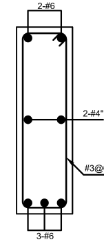
B-2 (MID SPAN) (9"x 30")
