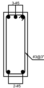
PB-1 (END SPAN) (9"x 24")
