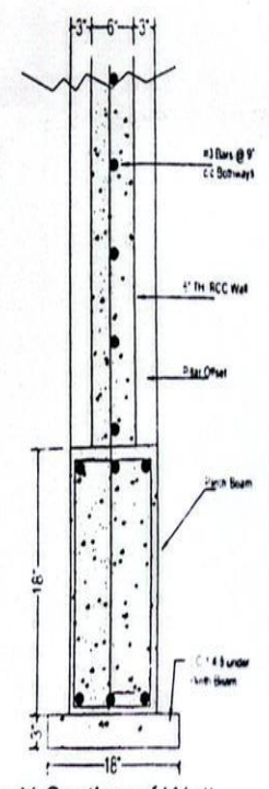
X-Section of Wall
