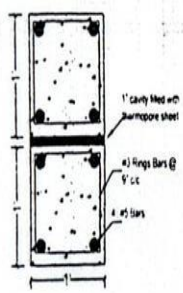
Double Column
