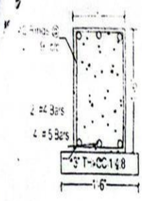
Plinth Beam
