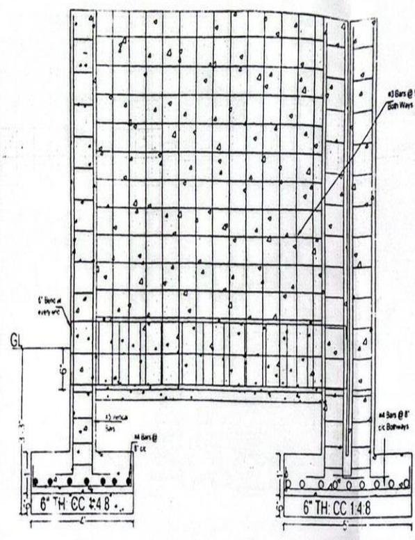
Elevation of Wall
