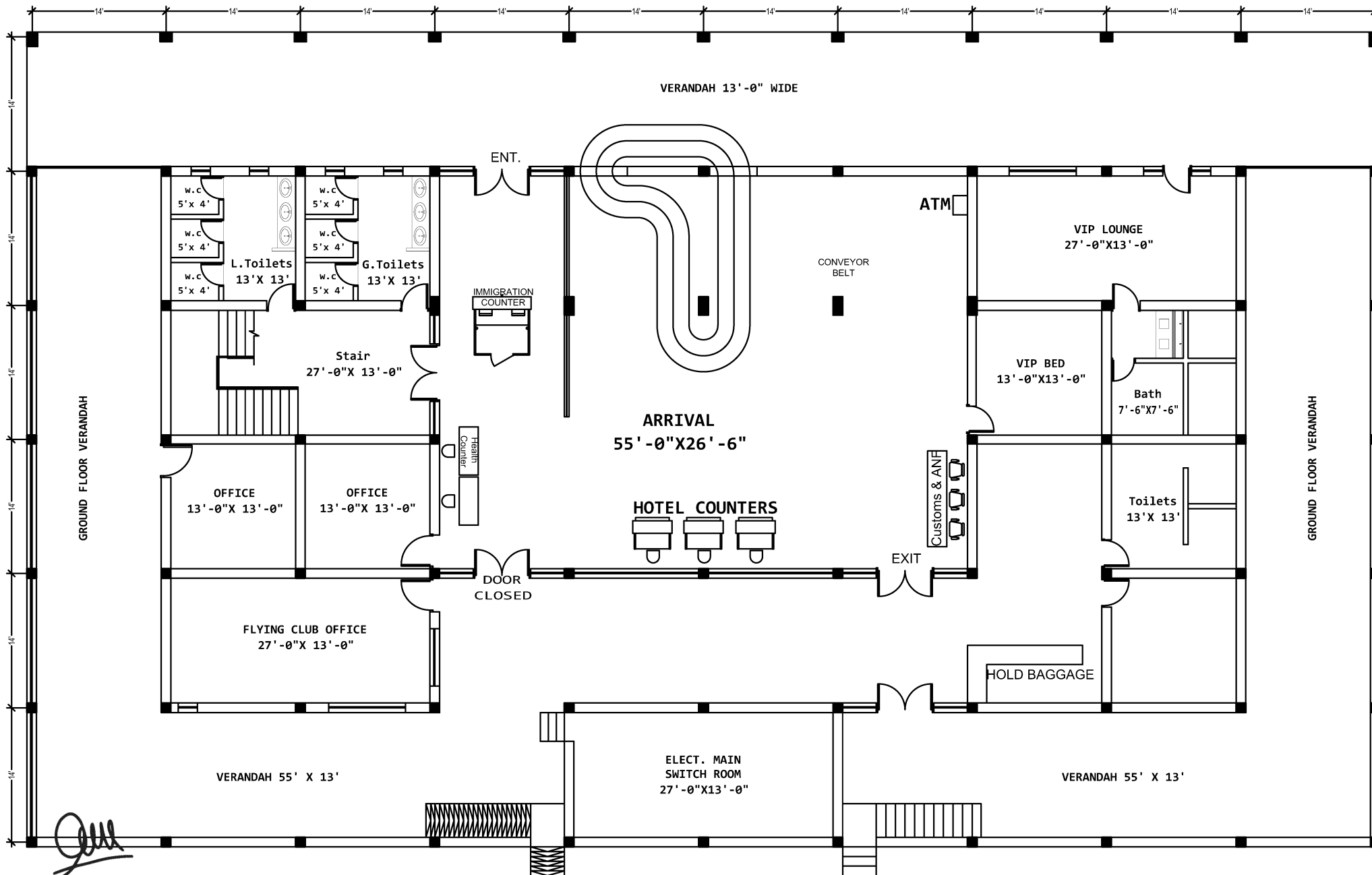
Hyderabad Terminal Building - GROUND FLOOR PLAN
