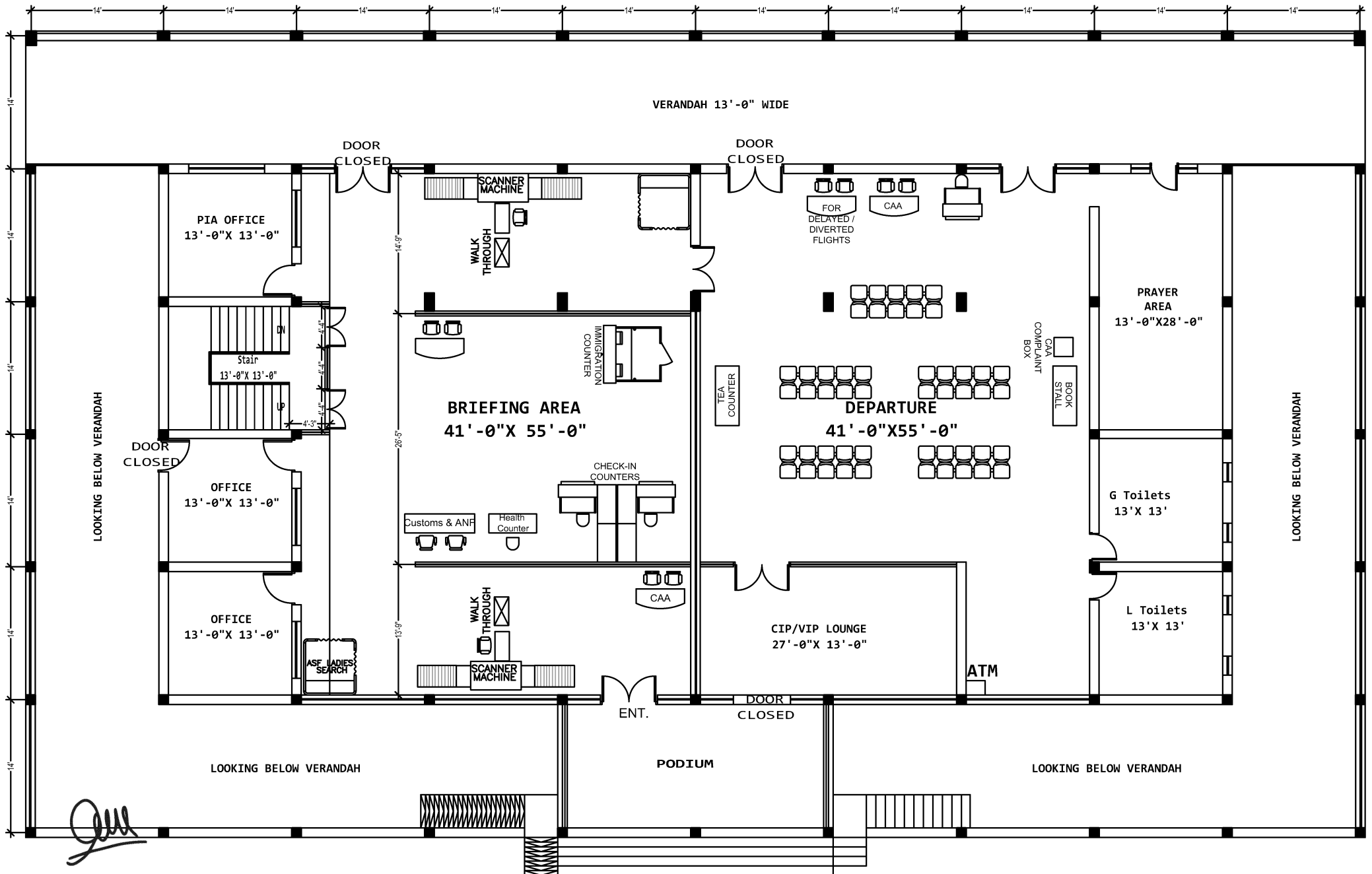
Hyderabad Terminal Building - FIRST FLOOR PLAN
