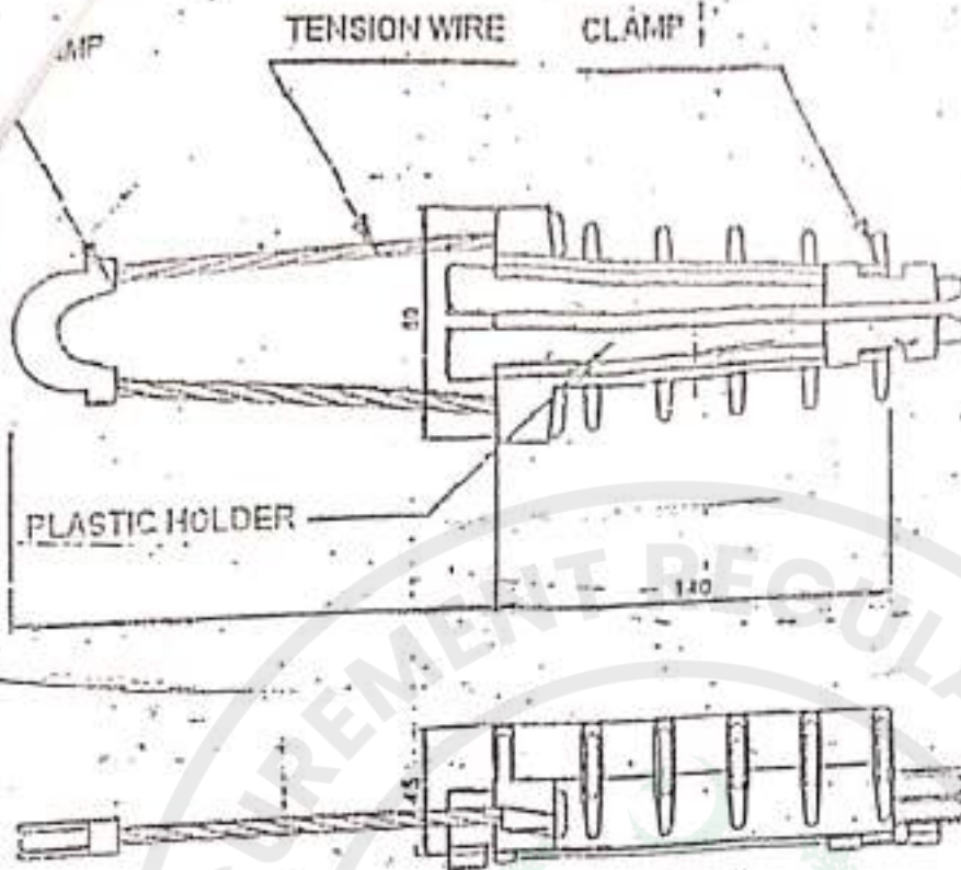
TENSION CLAMP ARRANGEMENT
