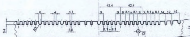
VIEW 'X'
