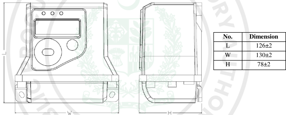
Figure - Dimensions of single phase meter
