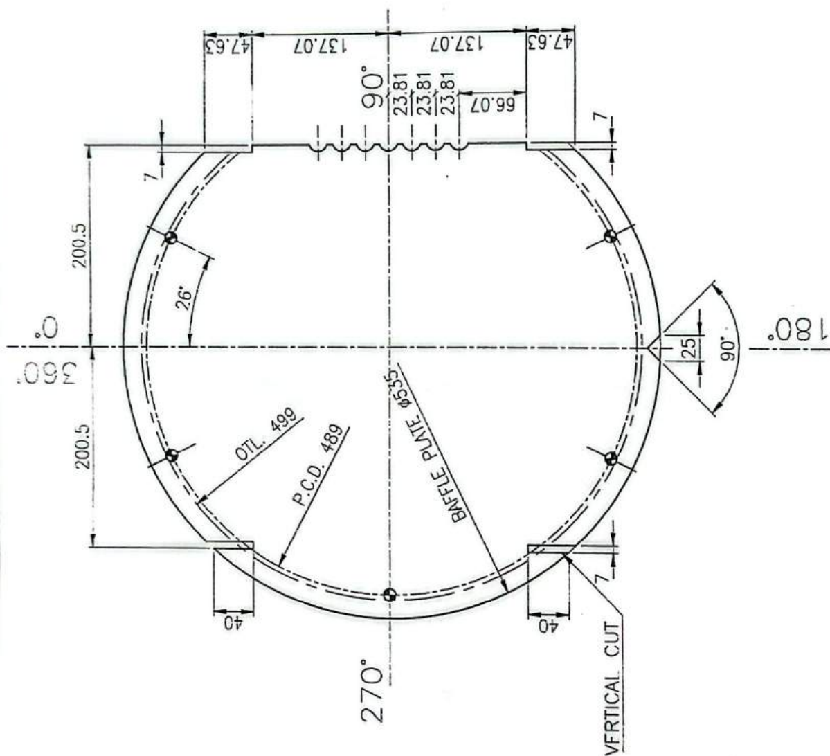
DETAIL OF BAFFLE PLATE
