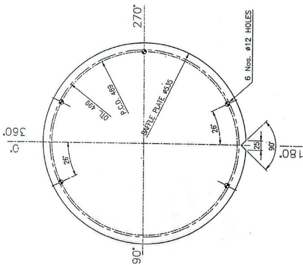
DETAIL OF SUPPORT PLATE
