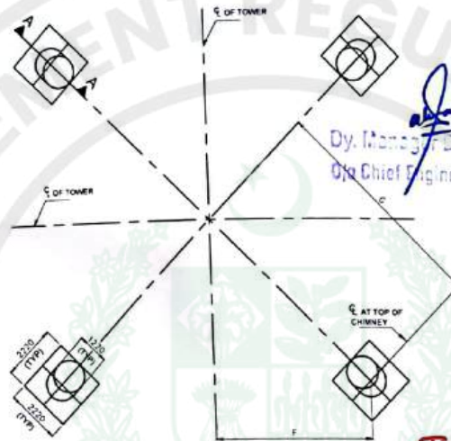
SETTING OUT FOUNDATION PLAN
