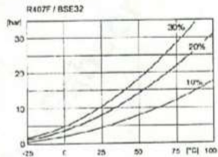
Fig. 2: Refrigerant pressure depending on the oil temperature and the refrigerant content (mass % of refrigerant in oil-refrigerant blend)
