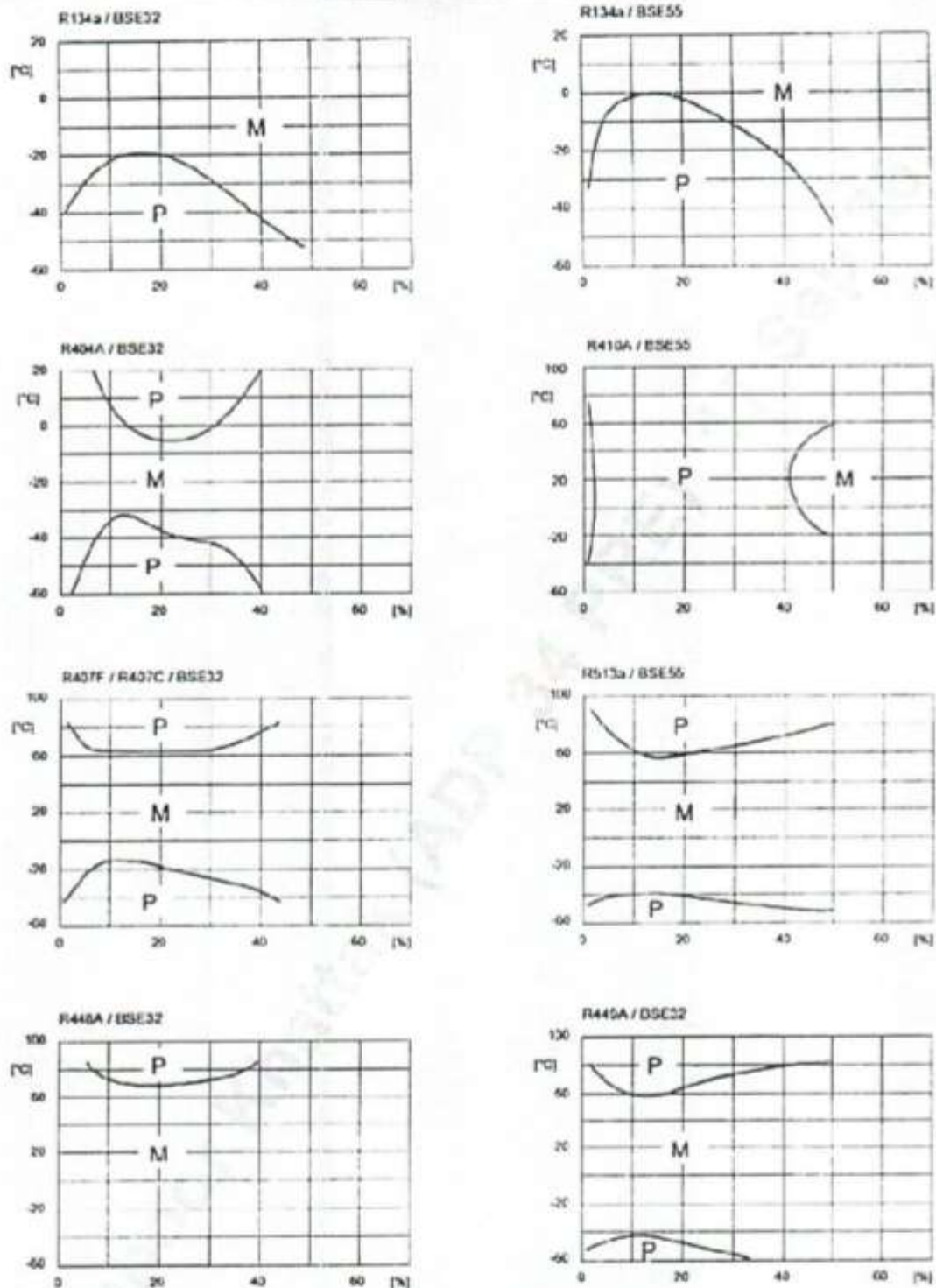
Fig. 1: Miscibility limits: Limit temperature depending on oil content (mass % of oil in oil-refrigerant blend)
