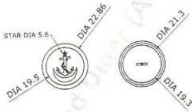
FRONT BUTTON DETAIL-5 (DIMENSION IN MM)
