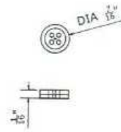
BUTTON DETAIL-4
