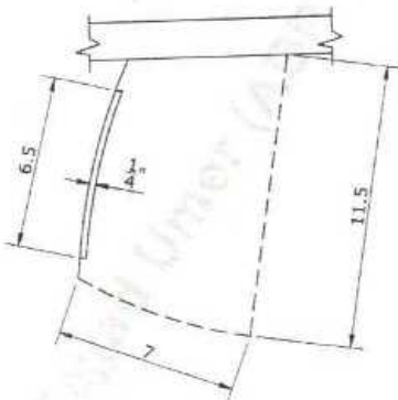
FRONT POCKET DETAIL-5
