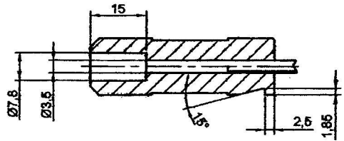
SEC: AA
