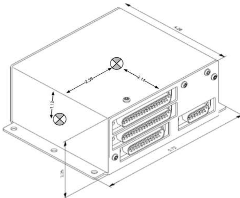
Figure 2-6 - ACU2 Outline Drawing (inches)
