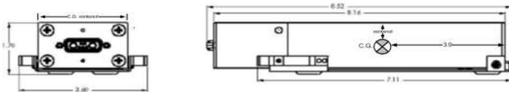
Figure 2-7 – EBB58 Emergency Backup Battery Drawing (inches)
