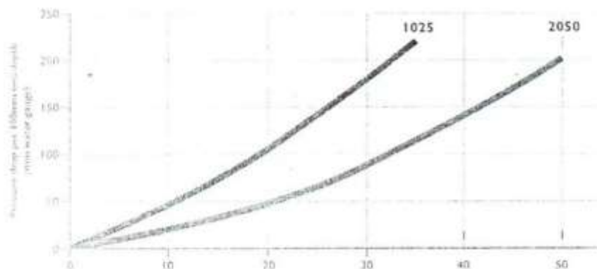
Air linear velocity - pressure drop relationship for 'L' and 'D' grade Sofnolime®
