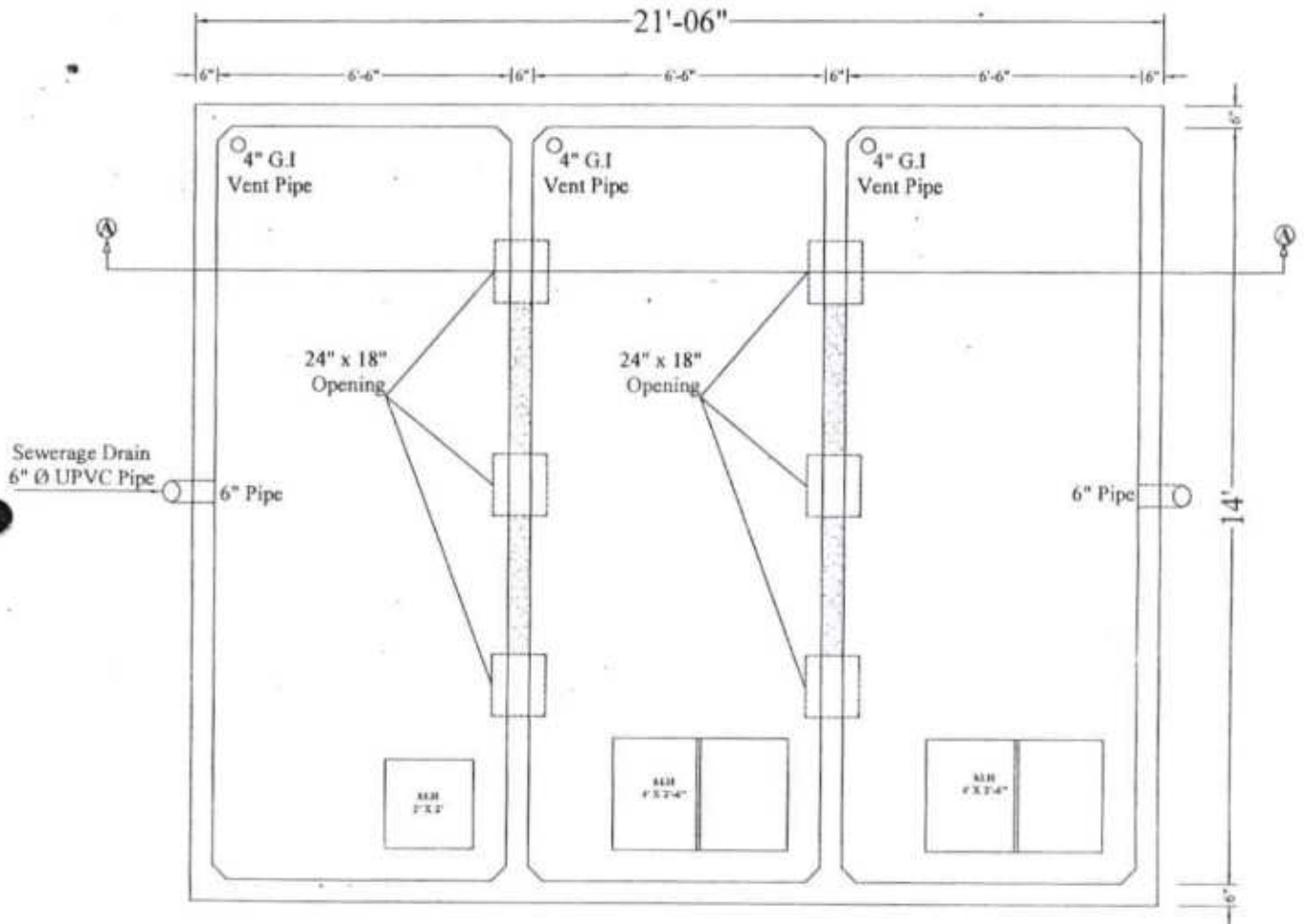
SEPTIC TANK PLAN
